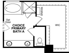
CHOICE PRIMARY BATH A
