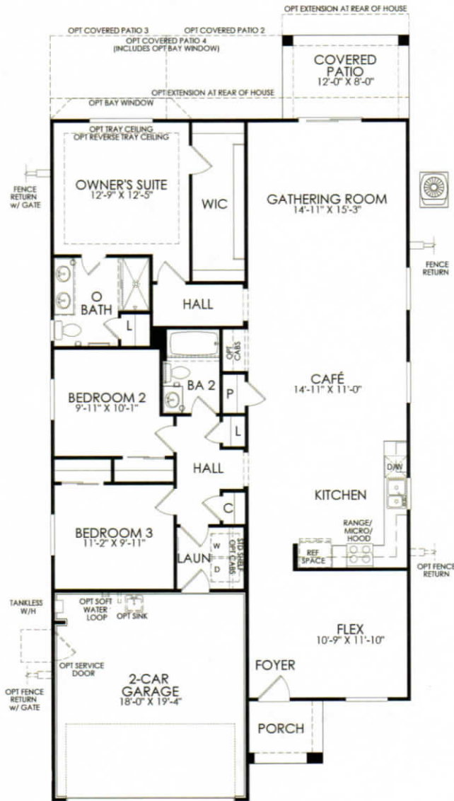
Floor Plan
