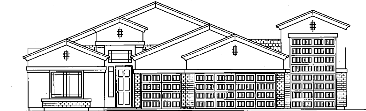
FRONT ELEVATION 'B'
