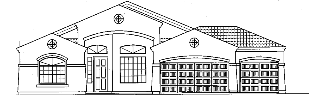
FRONT ELEVATION 'A'
