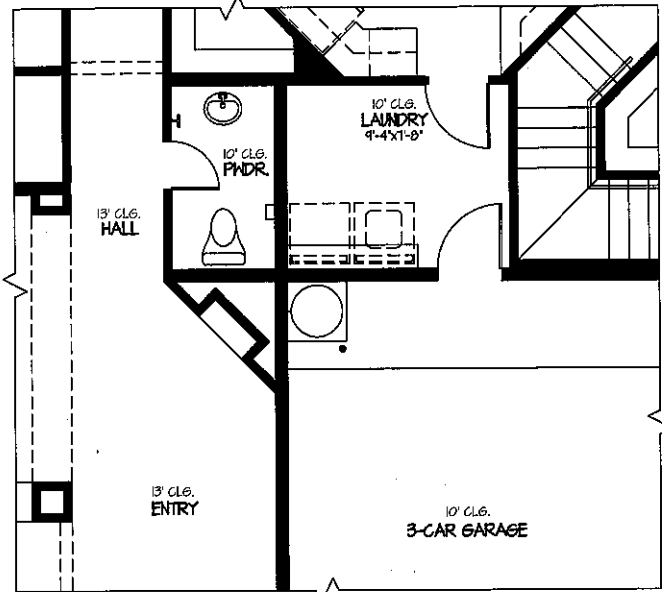
OPT. EXT. LAUNDRY W/ OPT. BASEMENT
