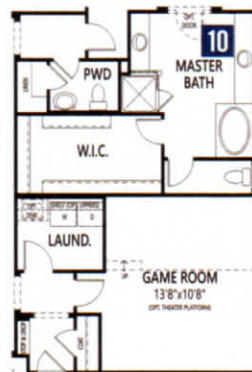
8 GAME ROOM IN LIEU OF TANDEM GARAGE (Additional 185 SQ.FT.)
