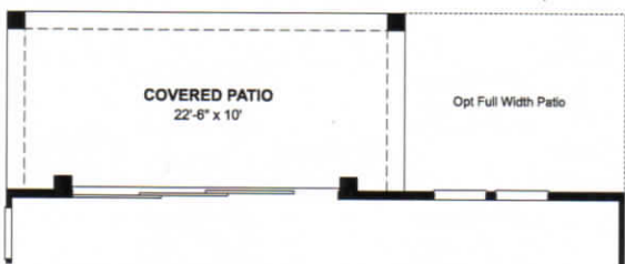
Opt 15' Sliding Glass Door w/ Extended & Full Width Covered Patio
