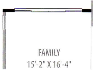
12ft Sliding Glass Doors at Family Room
