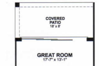
Opt 15' Sliding Glass Door at Great Room
