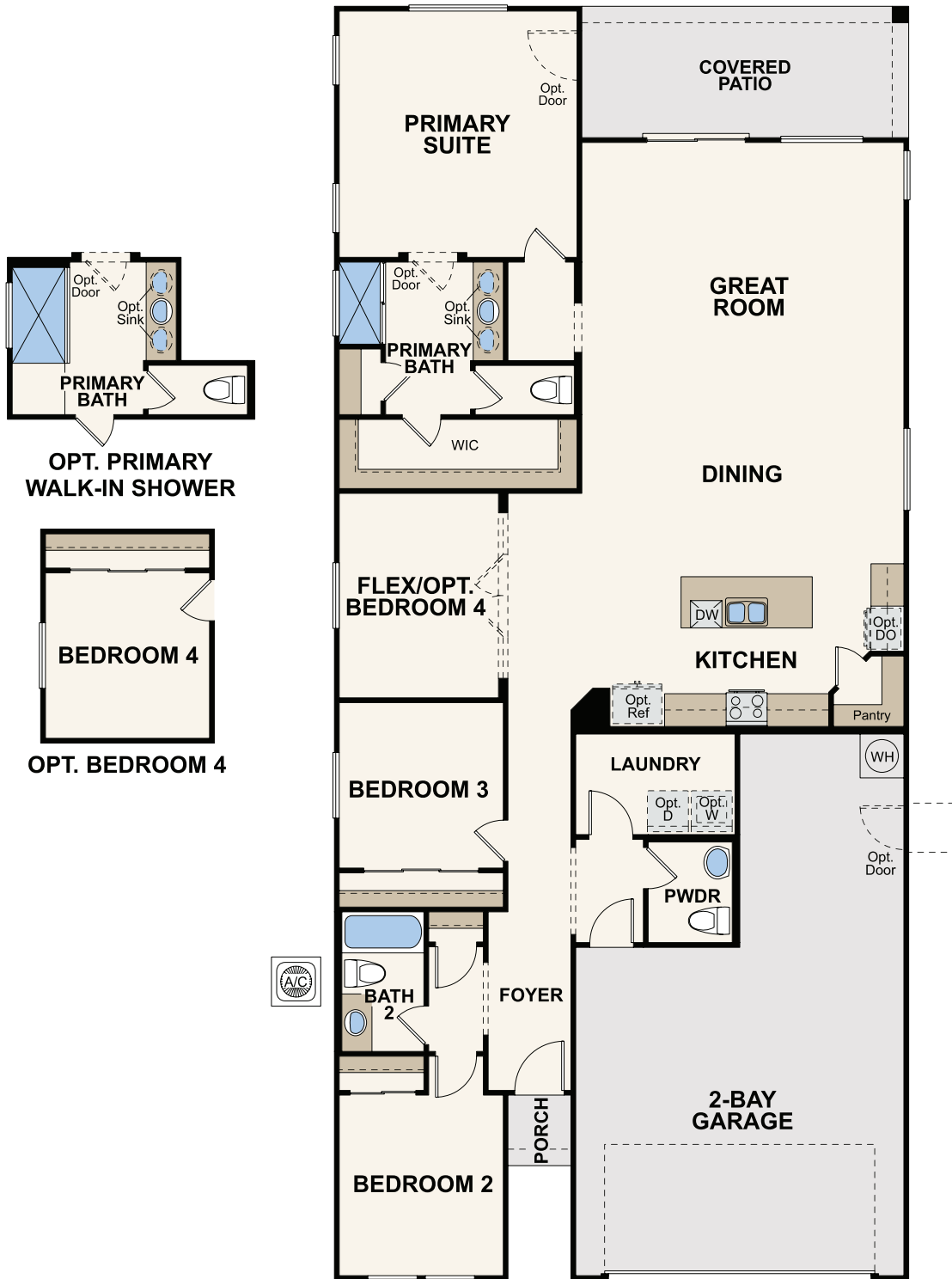
FLOOR PLAN
