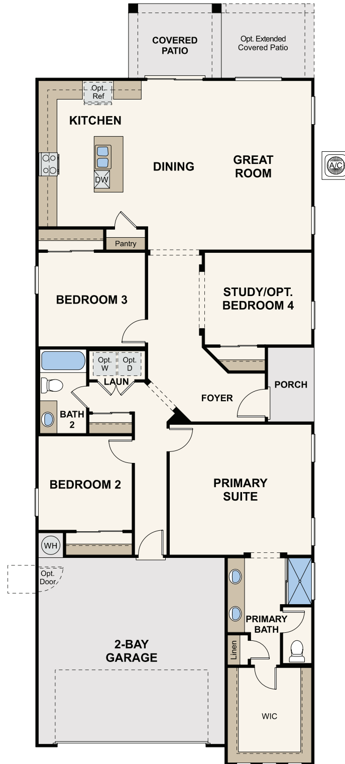
FLOOR PLAN
