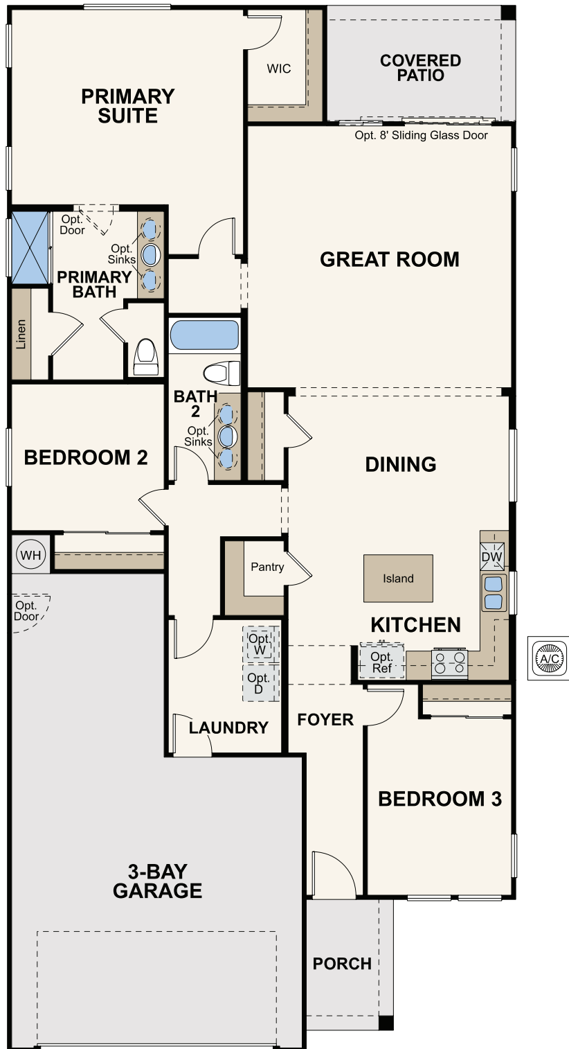
FLOOR PLAN
