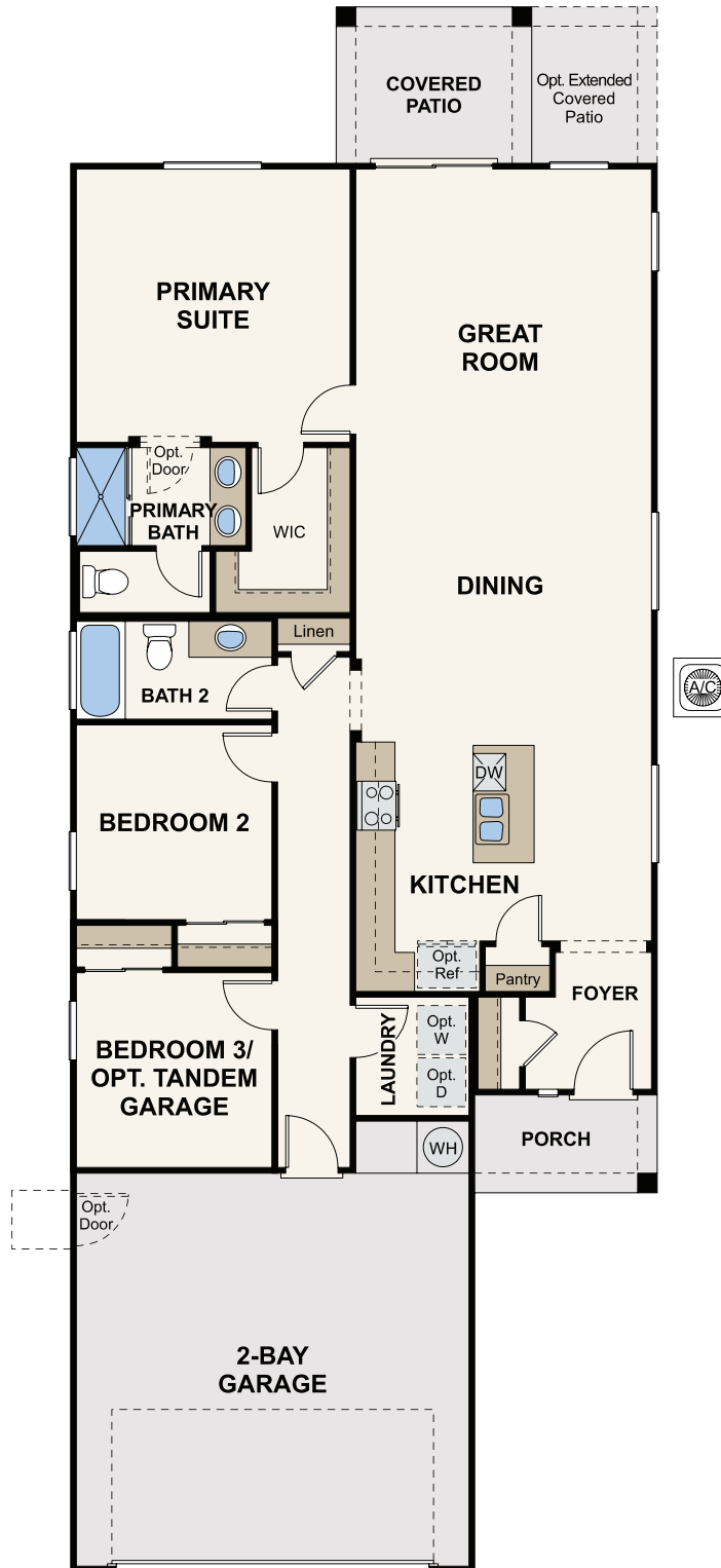
FLOOR PLAN
