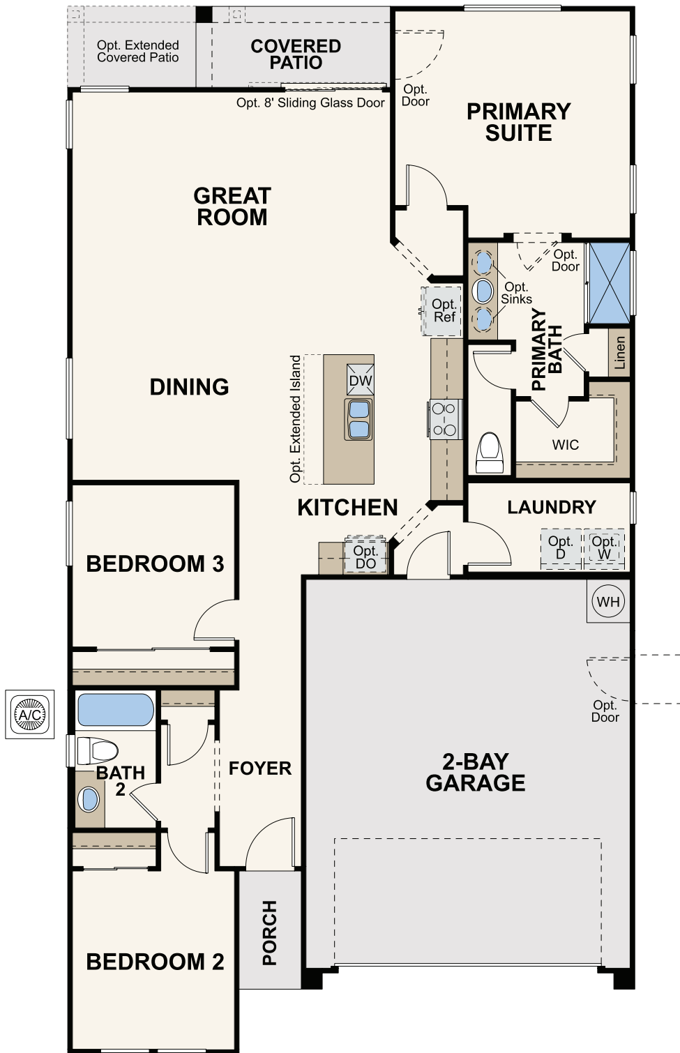
FLOOR PLAN
