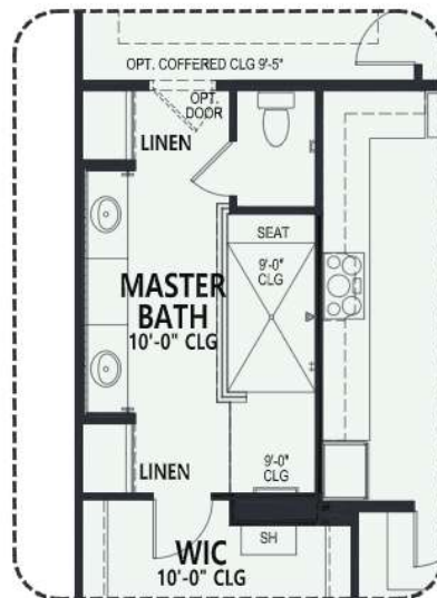
Opt. Curbless Shower
