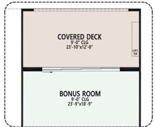
Opt. 16080 Stackable SGD at Second Floor Bonus Room
