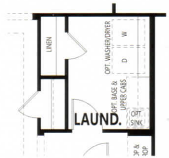
LINEN CLOSET AT LAUNDRY
