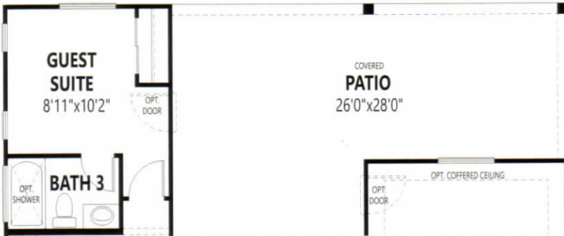
GUEST SUITE WITH BATH 3 AND EXTENDED COVERED PATIO
