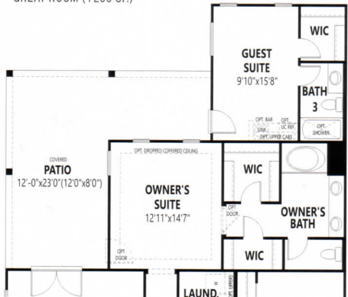
GUEST SUITE WITH BATH 3 AND EXTENDED COVERED PATIO WITH FRENCH DOORS AT GREAT ROOM (+256 SF.)
