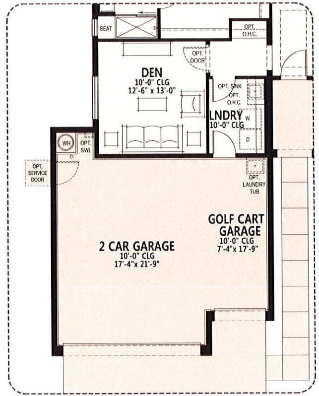
Opt. 3 ft. Expanded Den w/ Opt. Expanded Laundry w/ Opt. 4 ft. Garage Extension w/ Golf Cart Garage (55' Lot)
