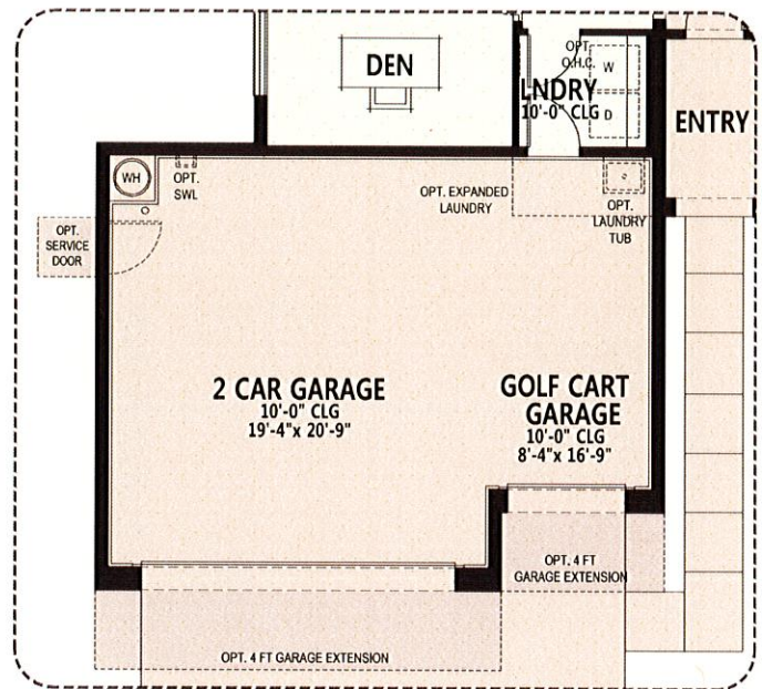
Opt. Golf Cart Garage (60' Lot)
