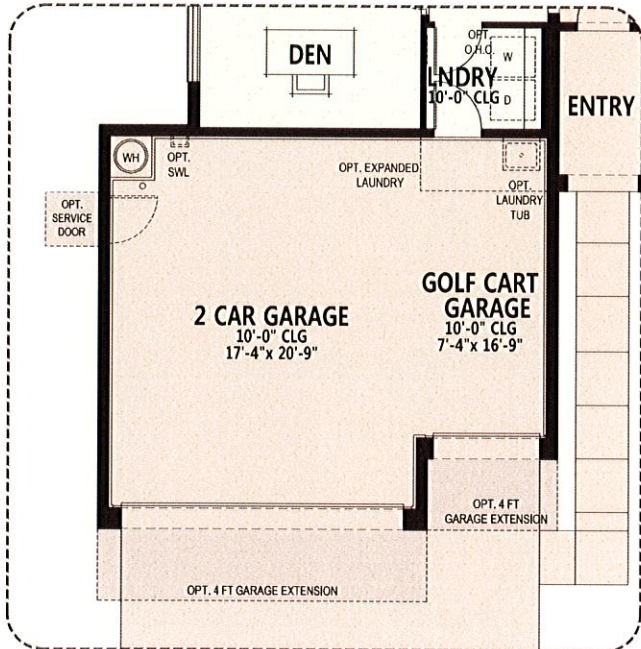
Opt. Golf Cart Garage (55' Lot)
