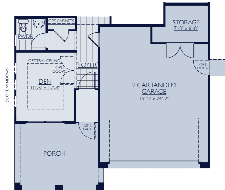
OPT. ENCLOSED STORAGE WITH 4' GARAGE EXTENSION
