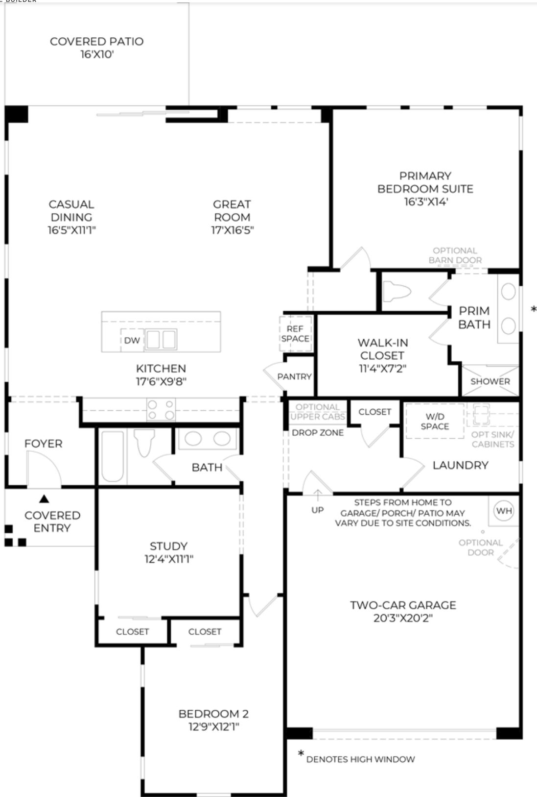
Floor Plan 10' CEILING HEIGHT
